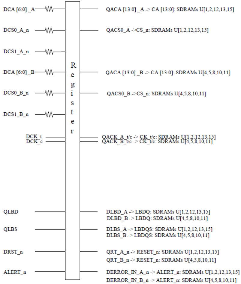
Figure 1 - Function Block Diagram_SCA16GR03H1F1C-56B
