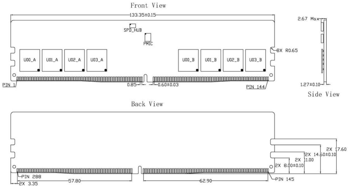
Figure 2 - Package Dimensions_SCA16GU03C2F1C-56B
