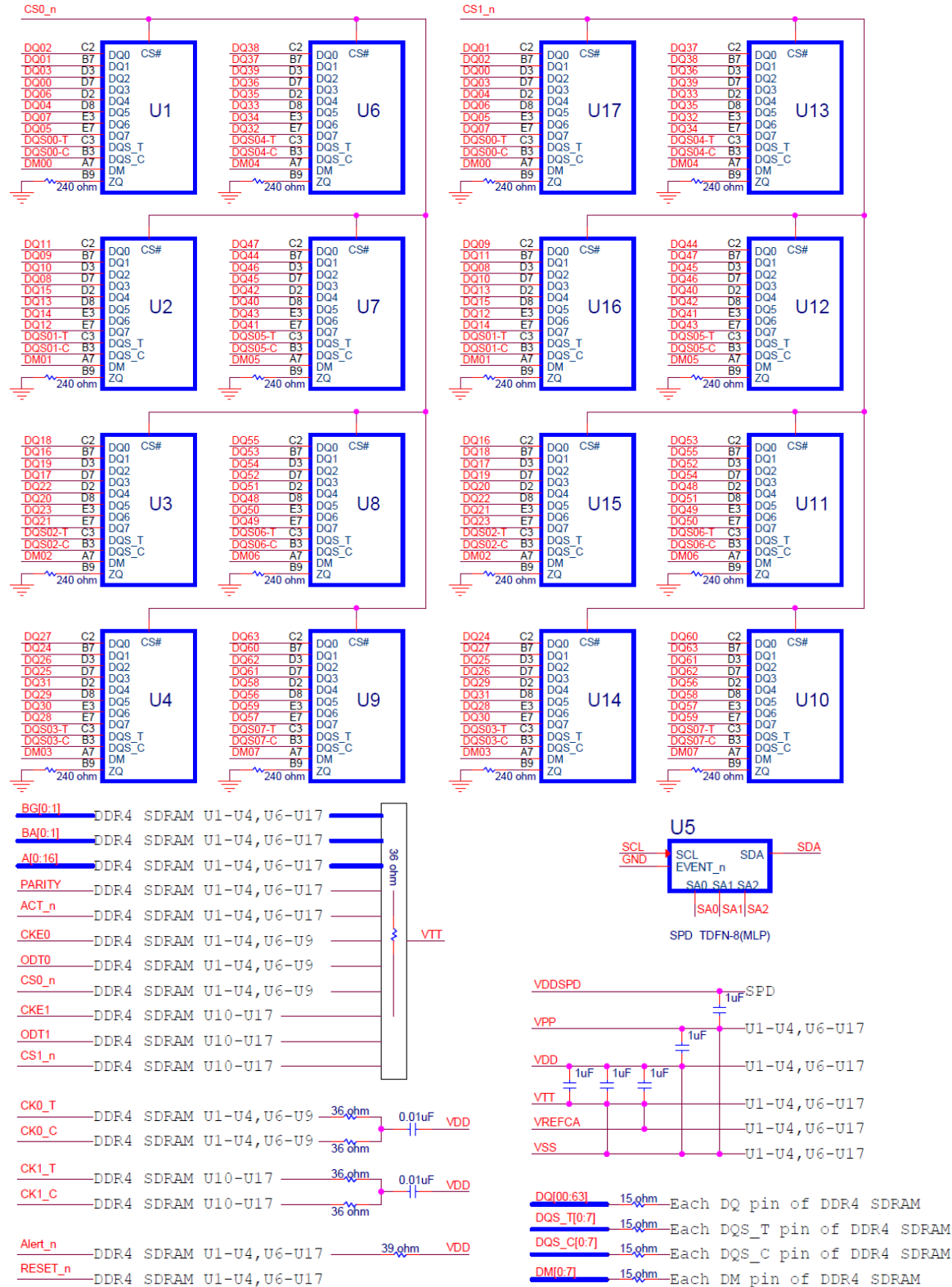
Figure 1 – Function Block Diagram_SCC16GU13G2F1C-32AA
