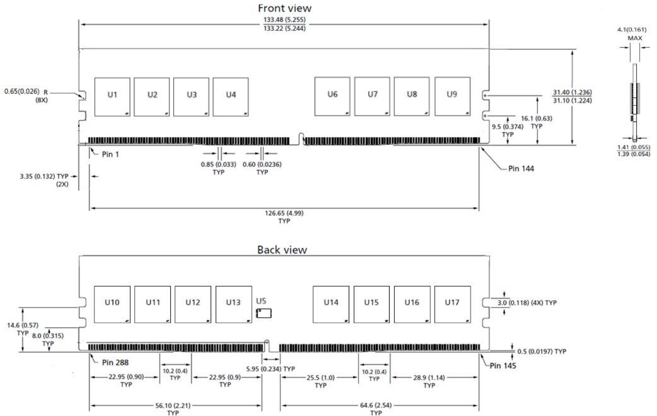
Figure 2 - Package Dimensions_SCC16GU13G2F1C-32AA
