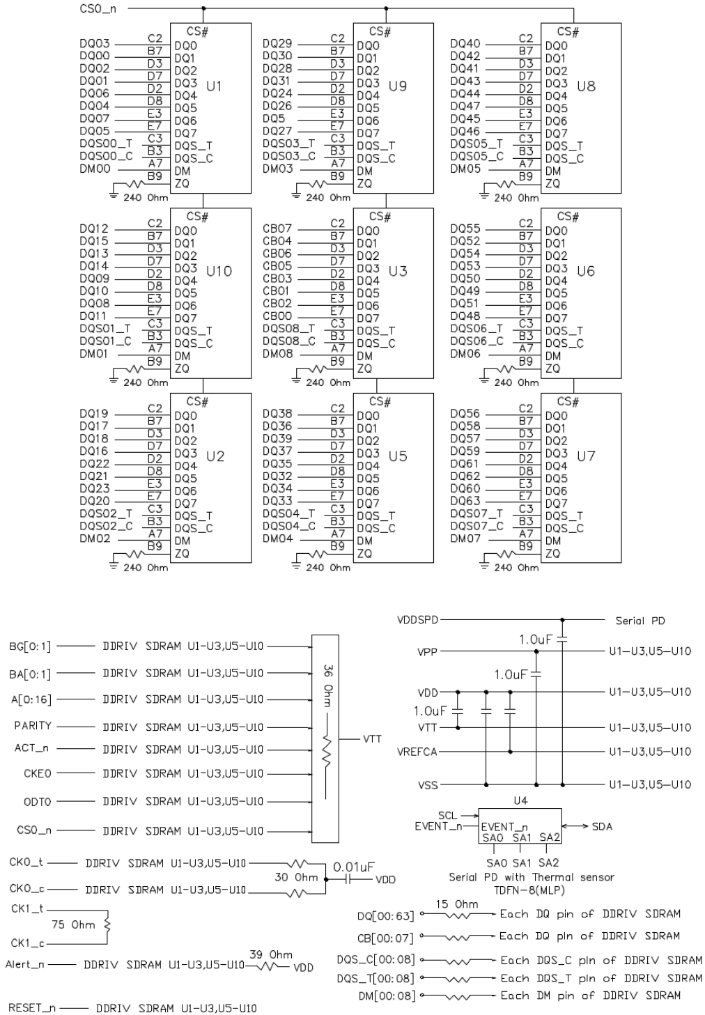
Figure 1 - Function Block Diagram_SCC08GX03C2F1C-32AA
