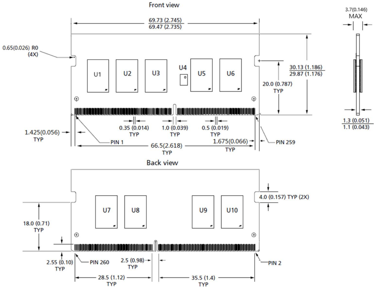
Figure 2 - Package Dimensions_SCC08GX03C2F1C-32AA
