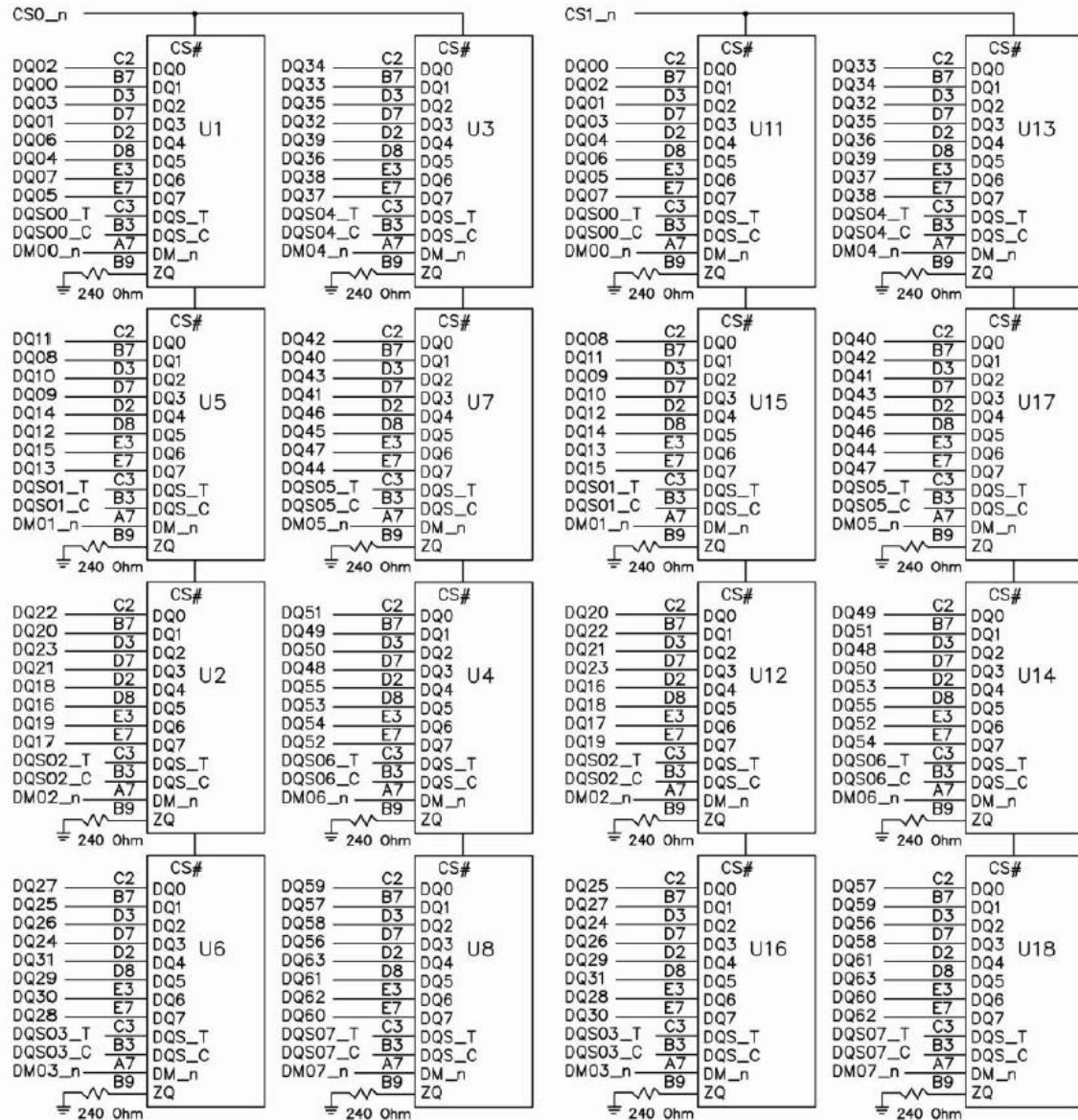
Figure 2 - Function Block Diagram_SCC32GS13H4F1C-32AA
