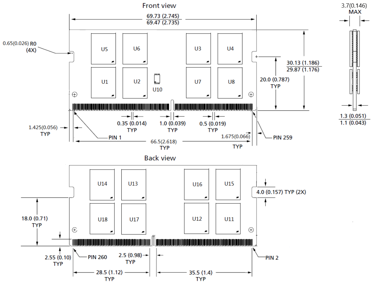
Figure 4 - Package Dimensions_SCC32GS13H4F1C-32AA
