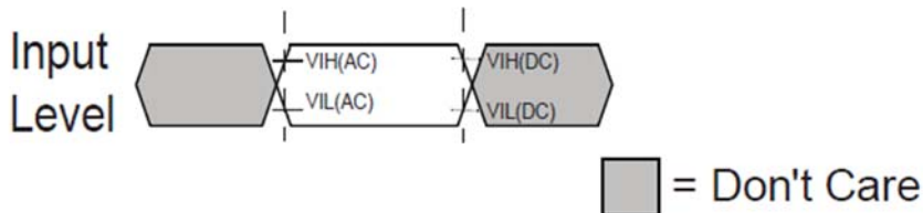
Figure 6 - Input Timing Definition for CKE
