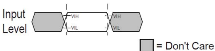
Figure 7 - Input AC Timing Definition for Reset_n and ODT_CA
