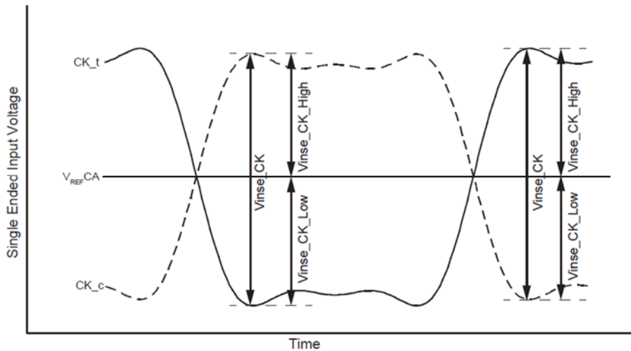
Figure 11 - Clock Single-Ended Input Voltage
