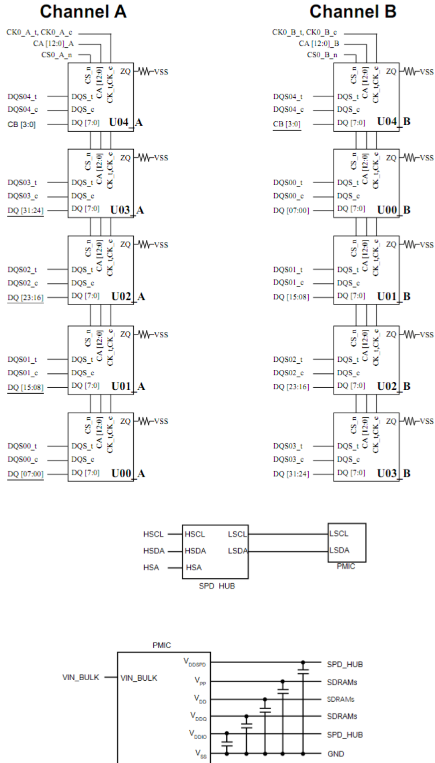
Figure 1 - Function Block Diagram_SCA16GE03H1F1C-56B
