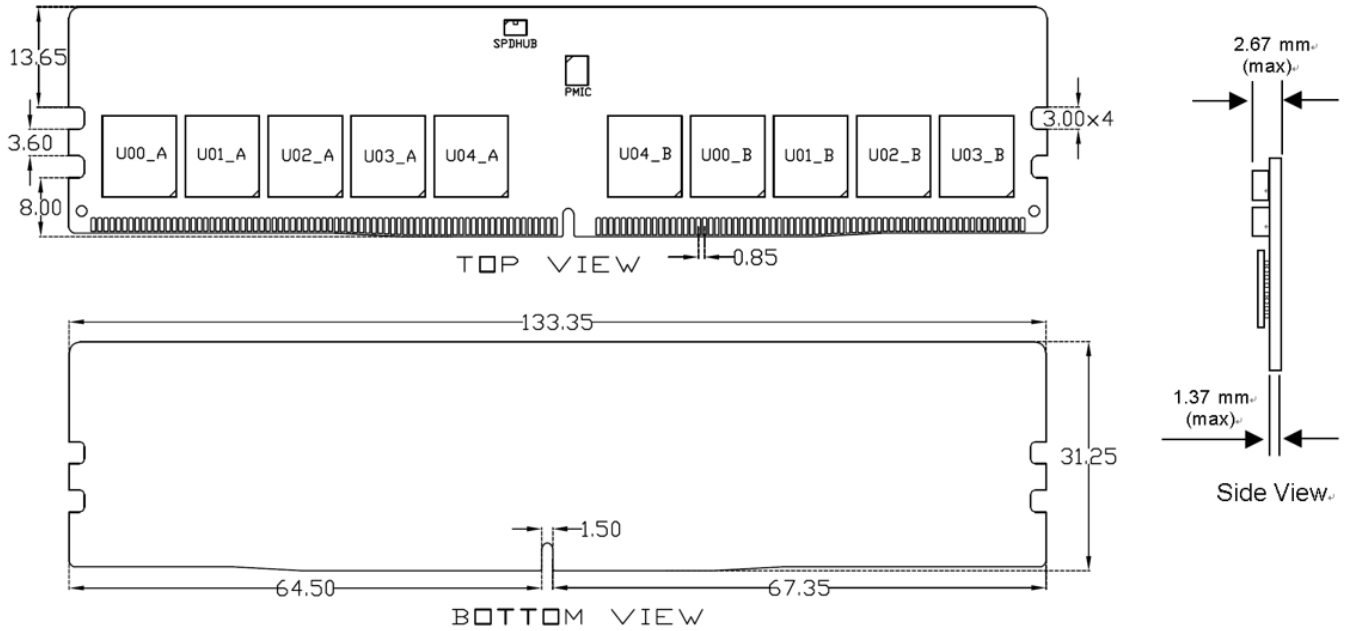
Figure 2 - Package Dimensions_SCA16GE03H1F1C-56B
