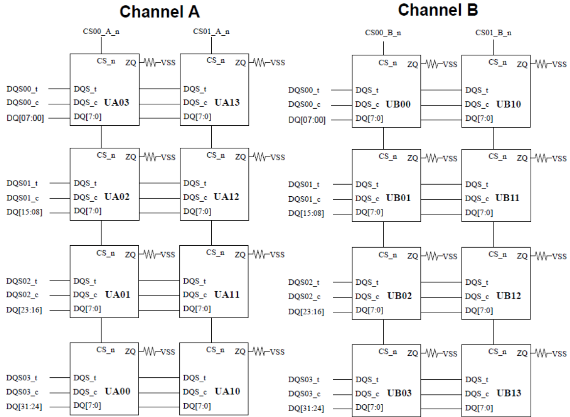
Figure 1 - Function Block Diagram_UCA32GU13A3F1C-48B
