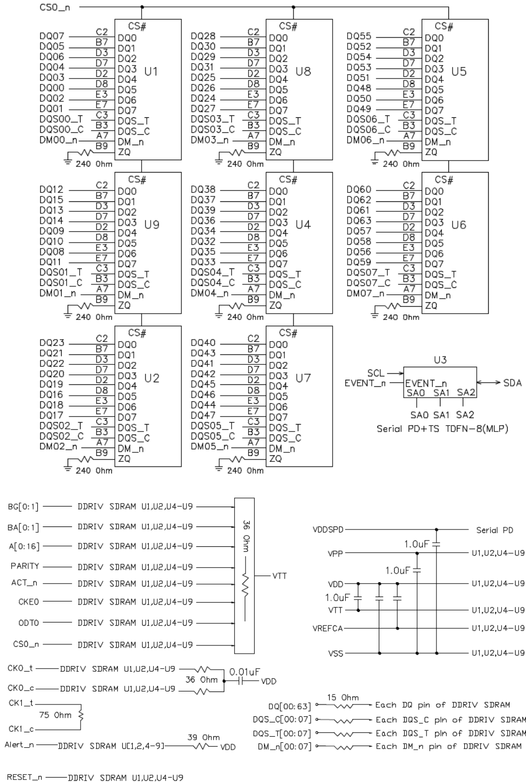
Figure 1 - Function Block Diagram_SCC16GS03C3F1C-32AA
