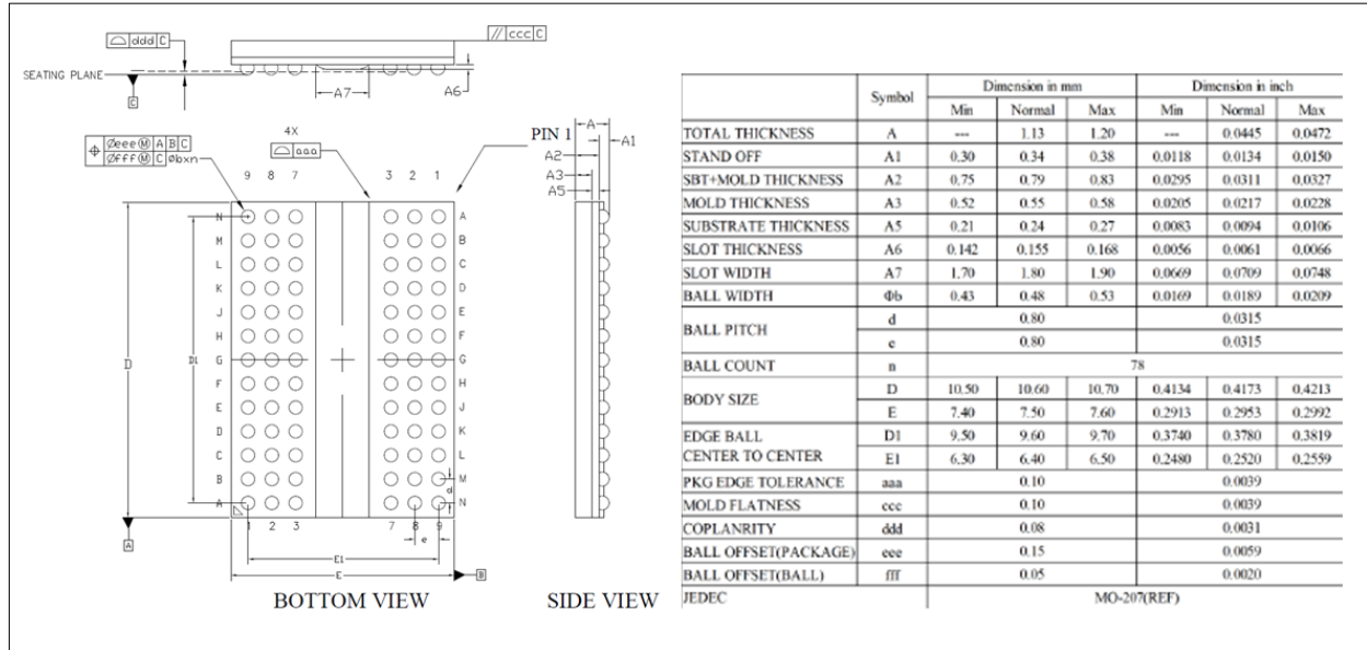
Figure 6 - Package outline for x8 Component
