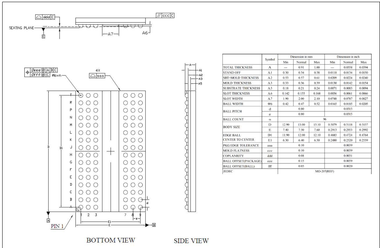
Figure 7 - Package outline for x16 Component
