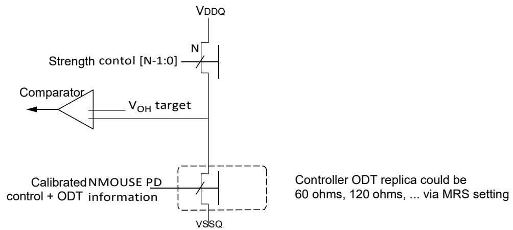
Figure 27- Pull-Up Calibration
