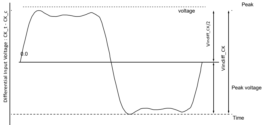
Figure 12-CK Differential Input Voltage
