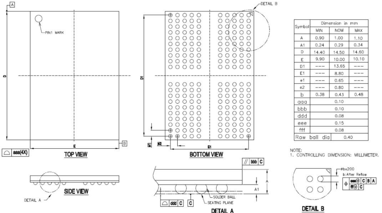
Figure 3-200-Ball TFBGA (10mm x 14.5mm x 1.1mm max)
