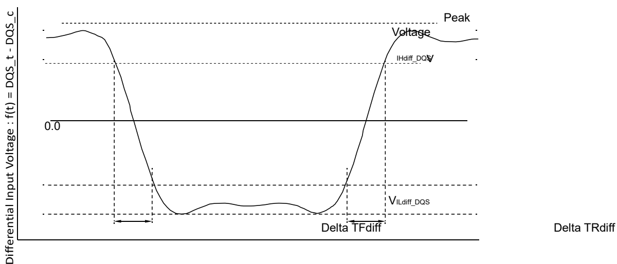
Figure 20-Differential Input Slew Rate Definition for DQS_t, DQS_c
