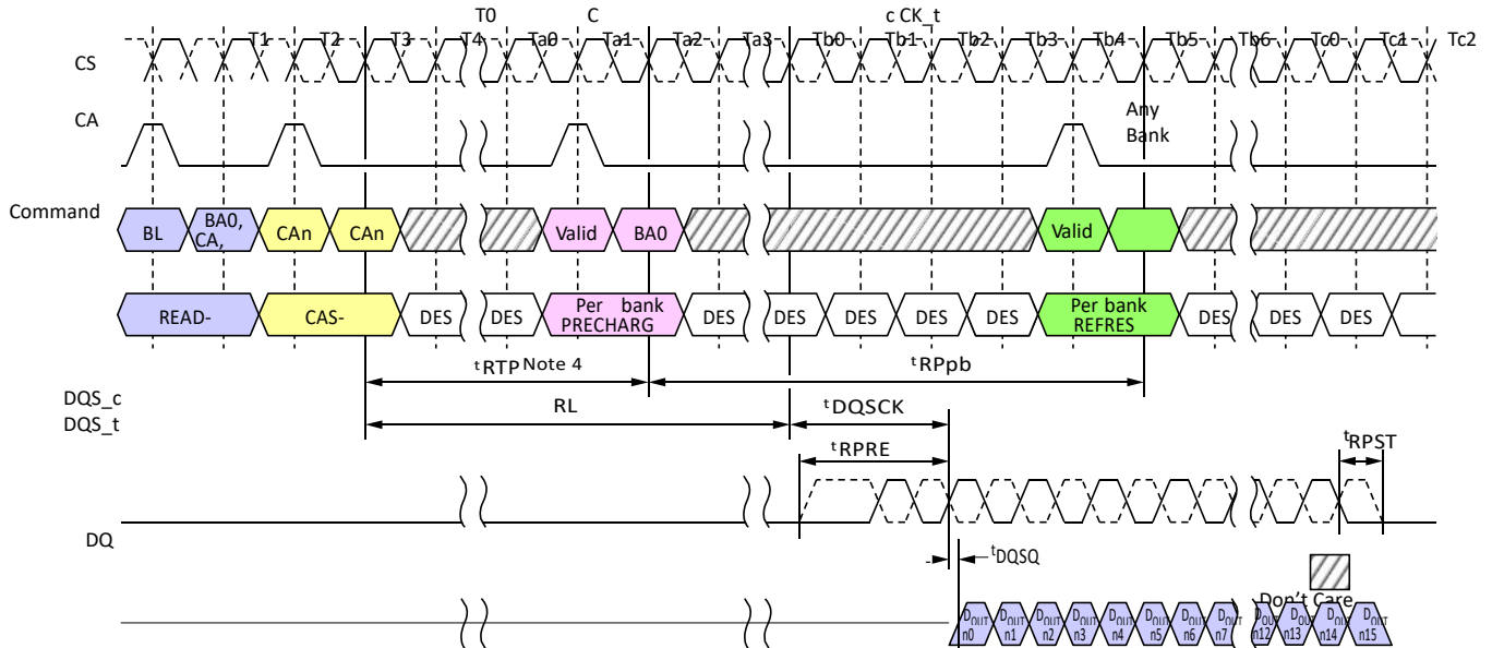
Figure 9-Burst READ Operation Followed by Per-Bank Refresh
