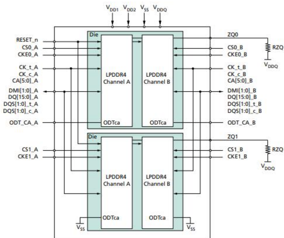
Figure 1-Dual-Die, Dual-Channel, Dual-Rank Package Block Diagram (x32 I/O)
