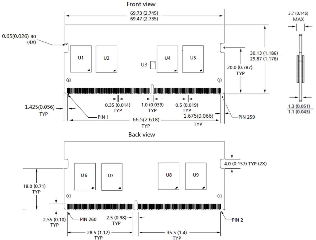
Figure 2 - Package Dimensions_SCQ16GS03M3F1C-32AA
