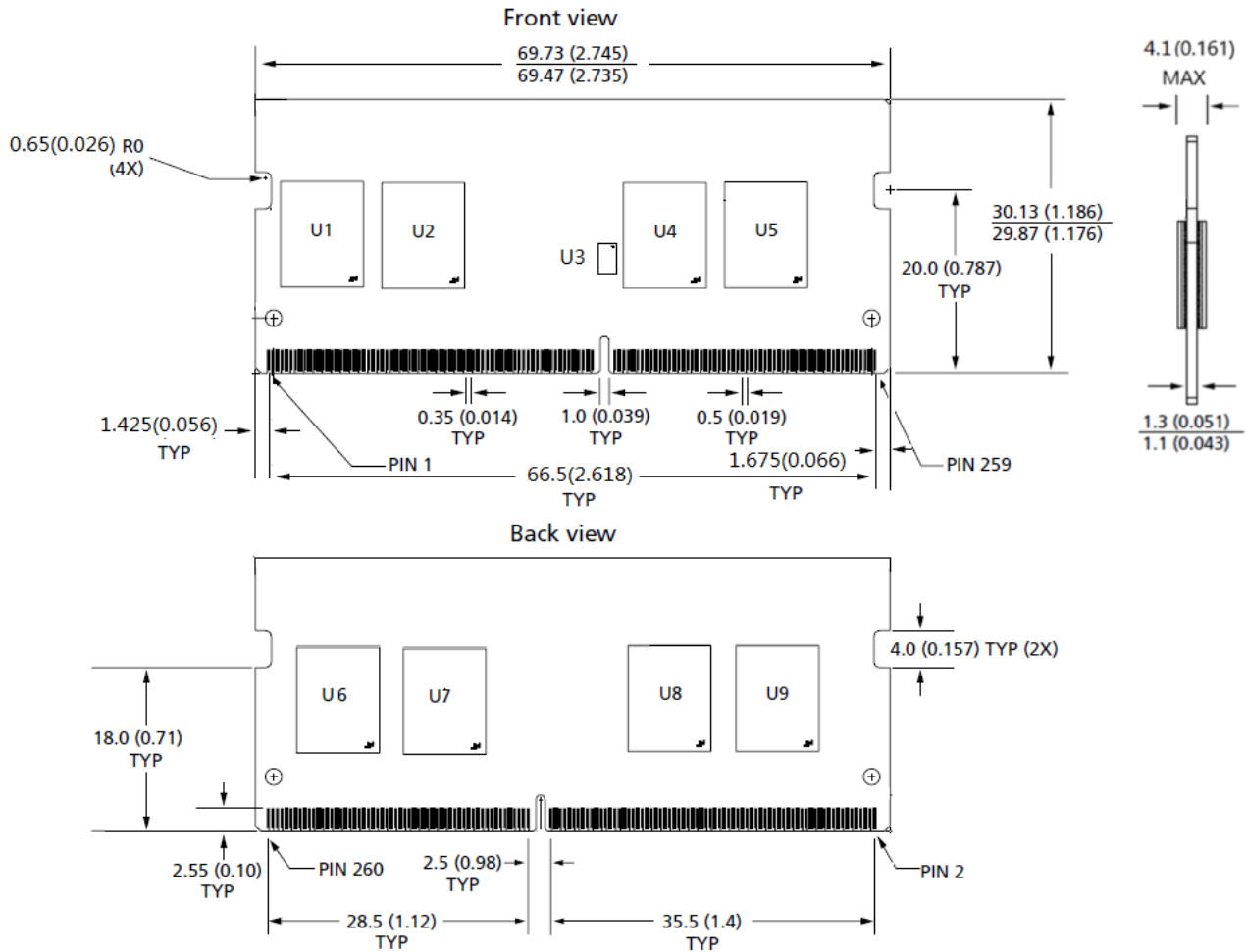
Figure 2 - Package Dimensions_SCQ08GS03M2F1C-32AA
