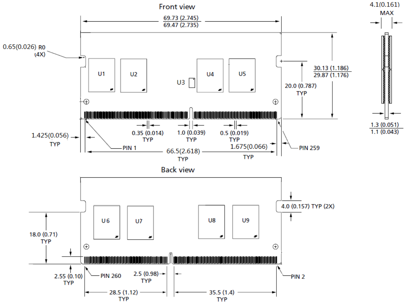
Figure 2 - Package Dimensions_SCQ16GS03M1F1C-32AA
