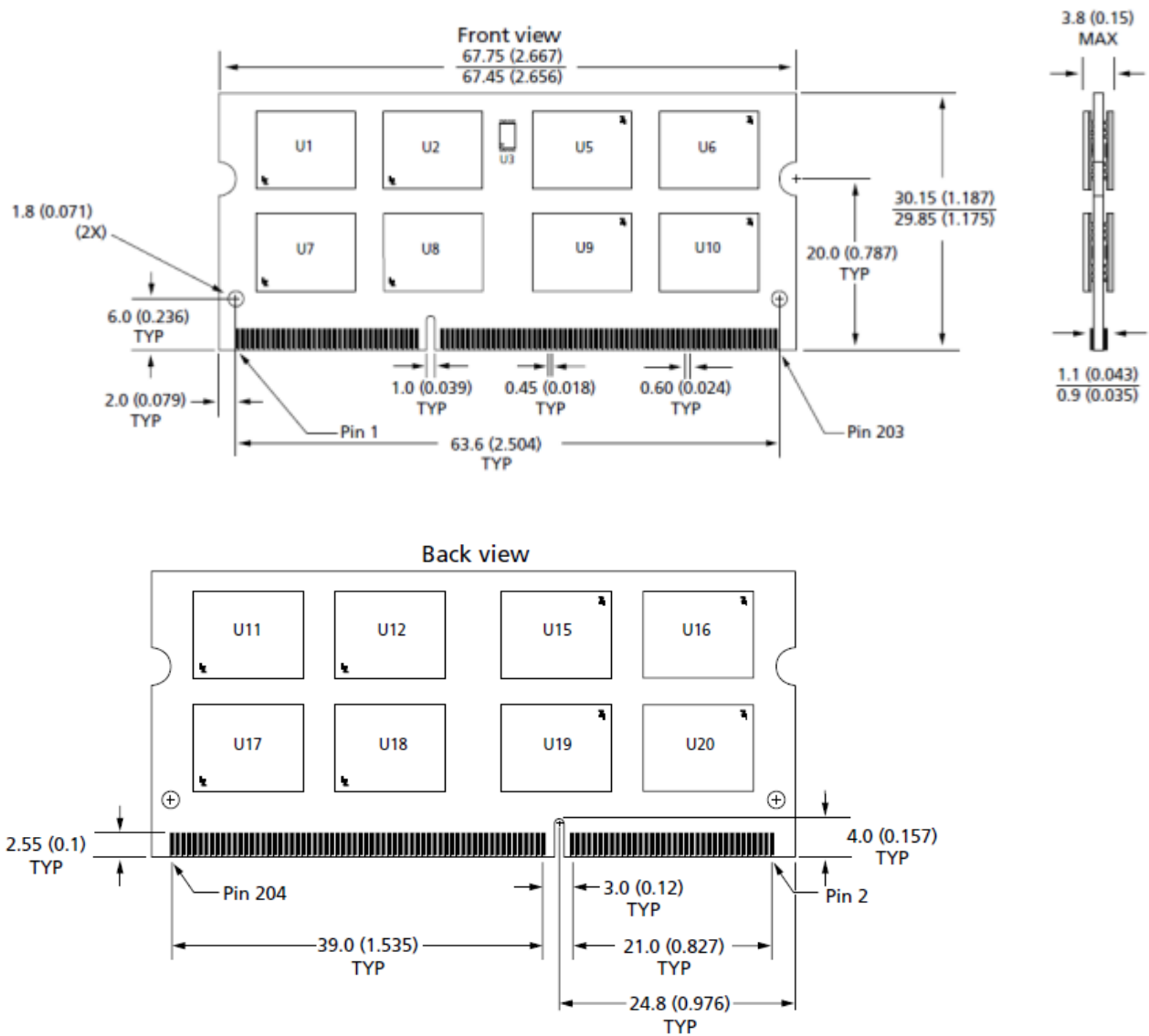
Figure 1 - Package Dimensions_ HXMSH8GS13A2F1CL16K
