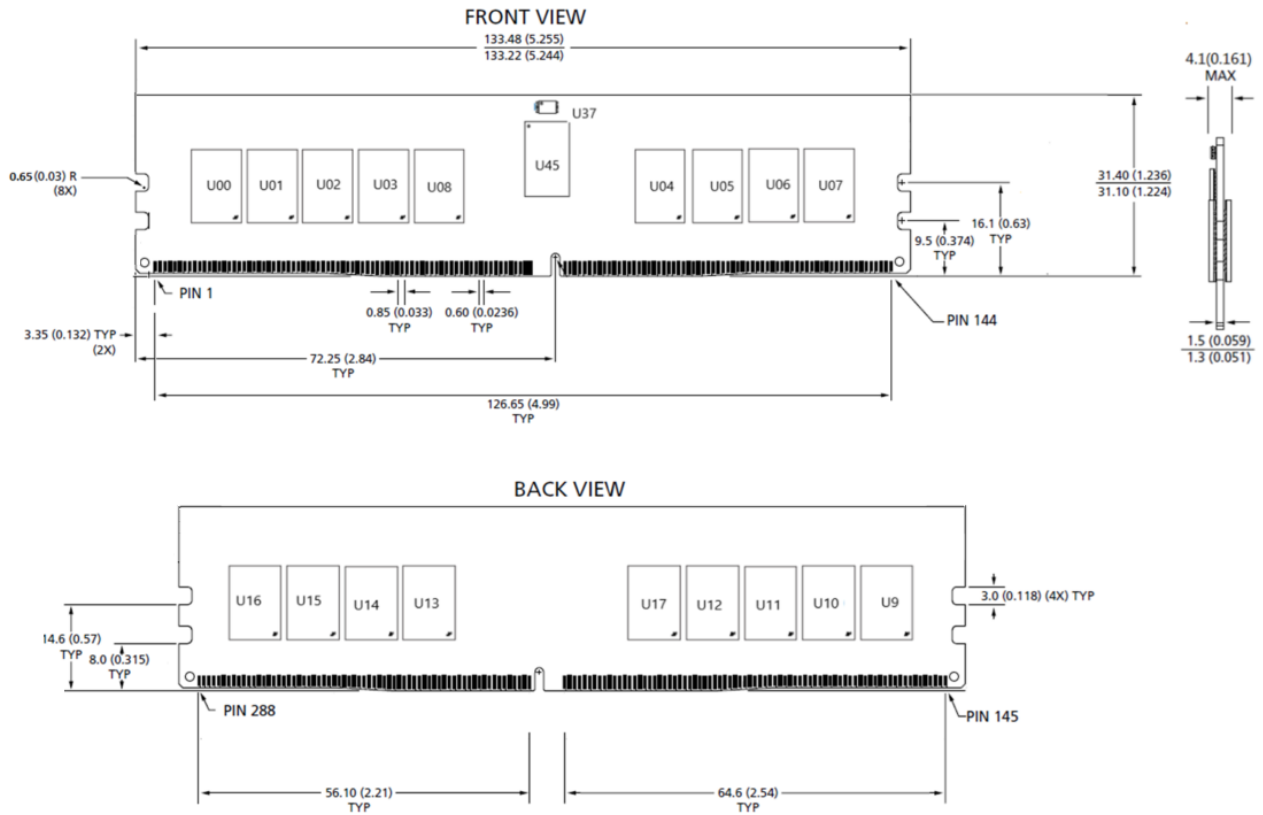
Figure 4 - Package Dimensions_SCQ32GP13M3F1C-32AA
