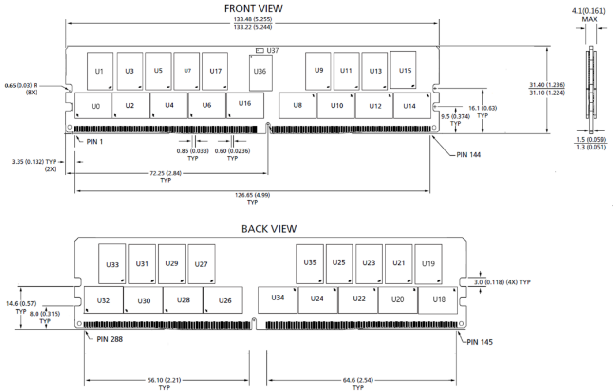
Figure 4 - Package Dimensions_SCC64GP12H4F1C-32AA
