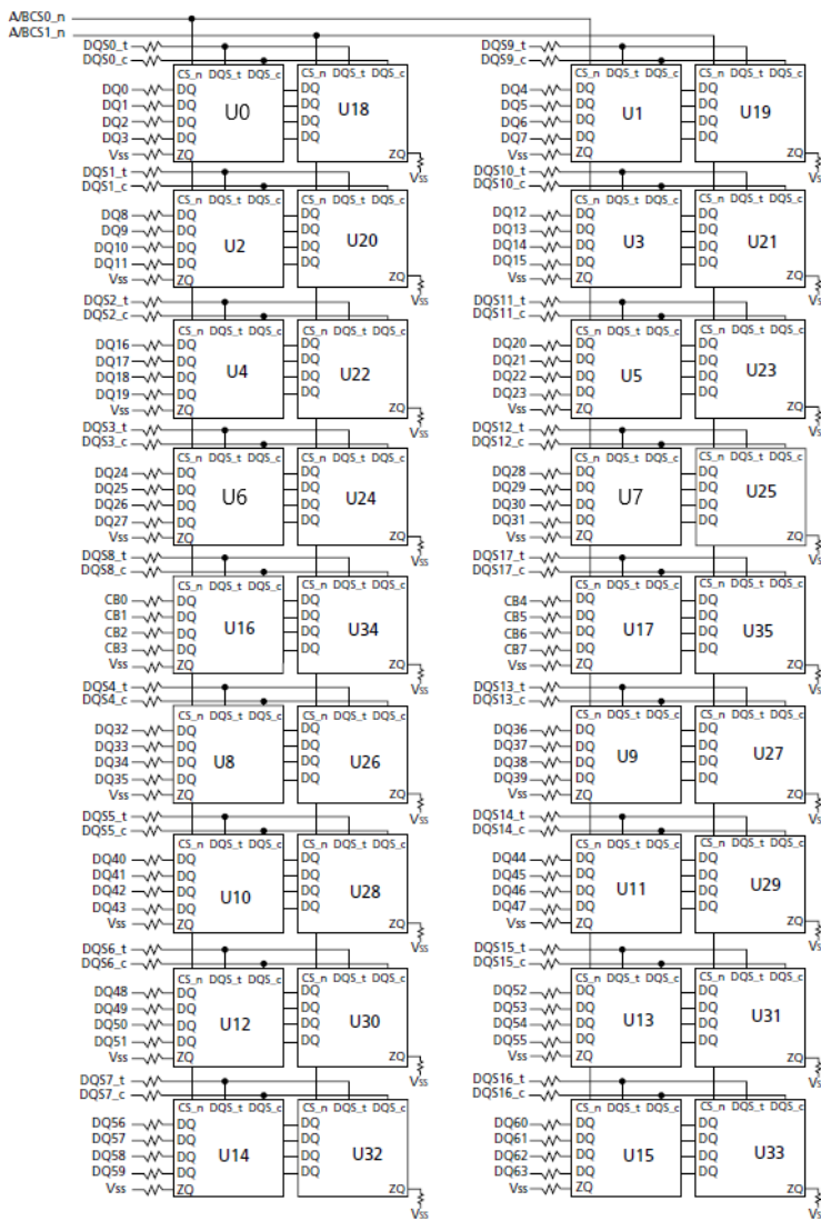
Figure 2 - Function Block Diagram_SCC64GP12H4F1C-32AA
