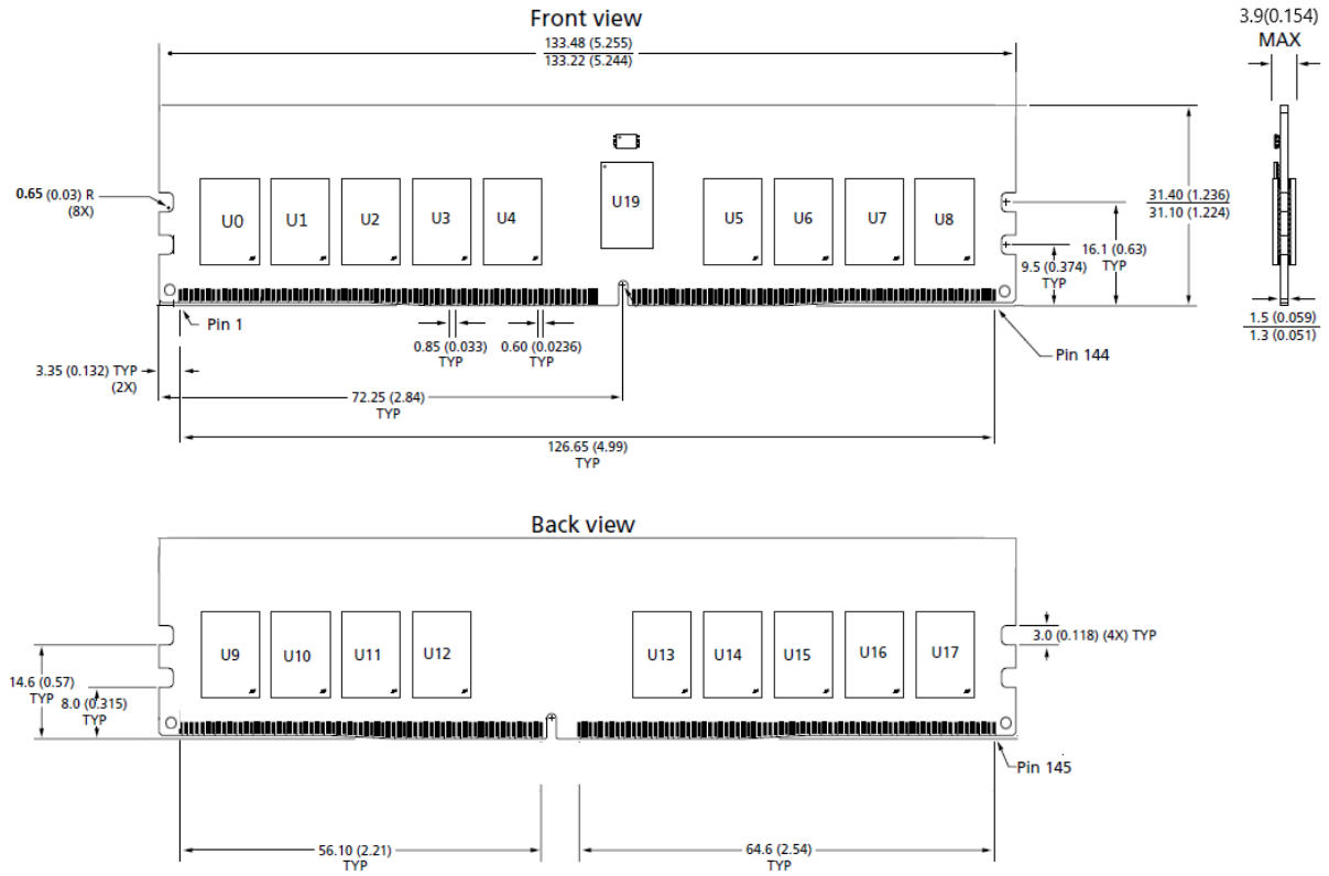
Figure 3 - Package Dimensions_SCC32GP02H4F1C-32AA
