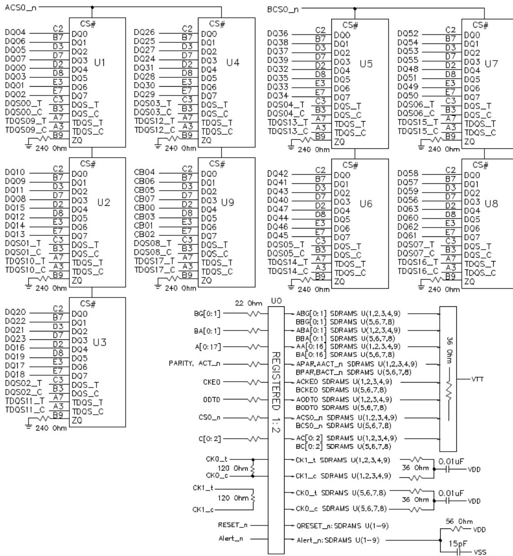
Figure 1 - Function Block Diagram_SCC16GP03H2F1V-32AA
