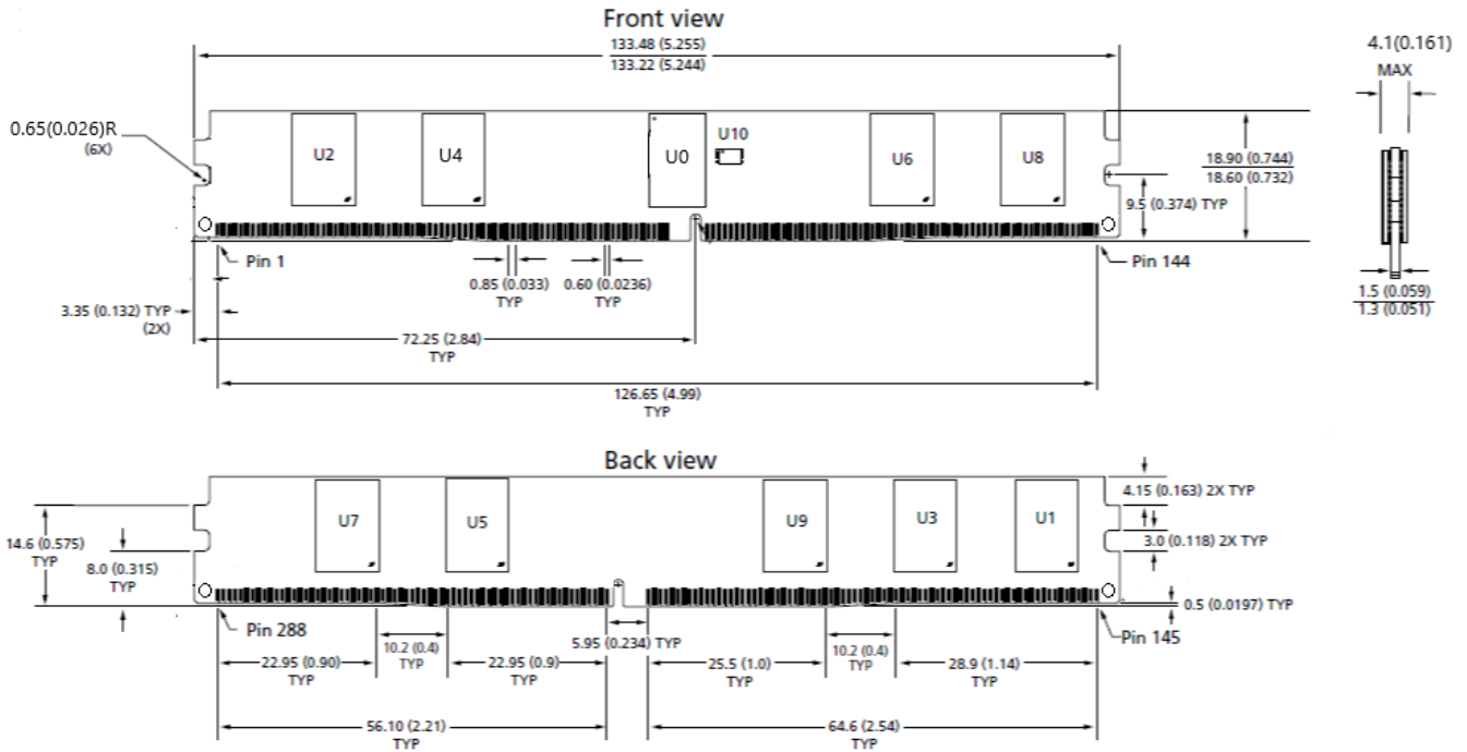
Figure 2 - Package Dimensions_SCC16GP03H2F1V-32AA
