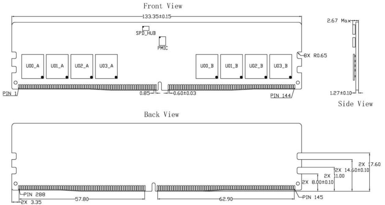
Figure 2 - Package Dimensions_SCA16GU03M1F1C-48B
